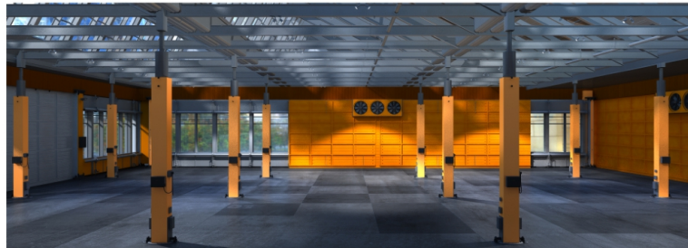
D3D-EnvFact-01-3
