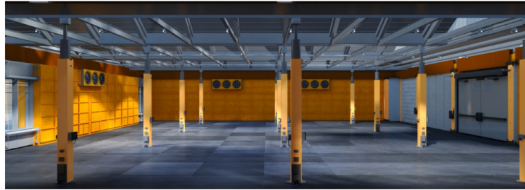
D3D-EnvFact-01-1
