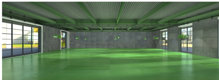
D3D-EnvFact-05-2
